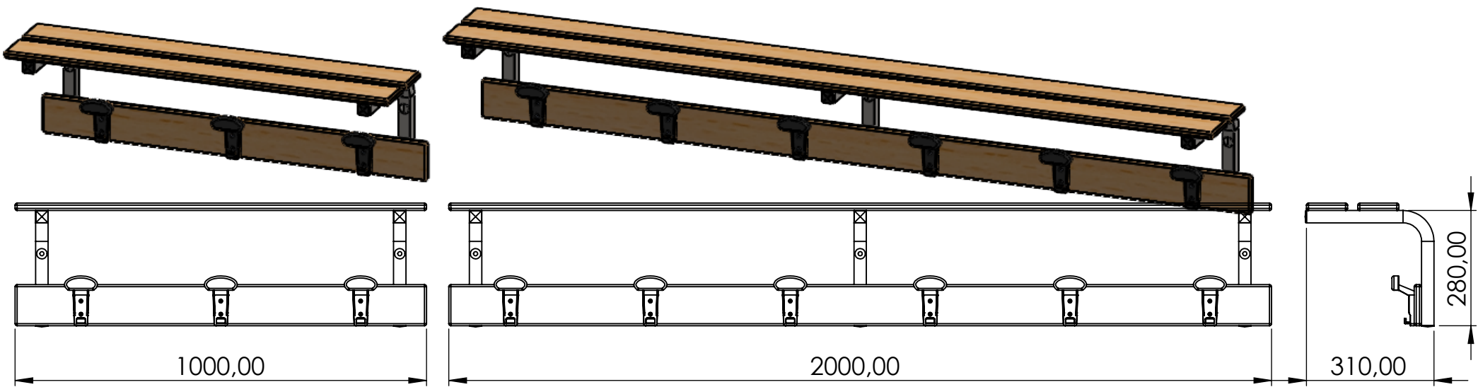
APPENDIABITI CON RIPIANO PORTABORSE - CLOTHES HANGER RAIL WITH BAG SHELF
