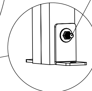
VITE TE M8x90 SCREW M8x90
