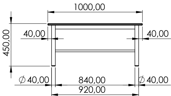
PANCA SPOGLIATOIO (SOLO SEDUTA) CHANGING ROOM BENCH (SEAT ONLY)
