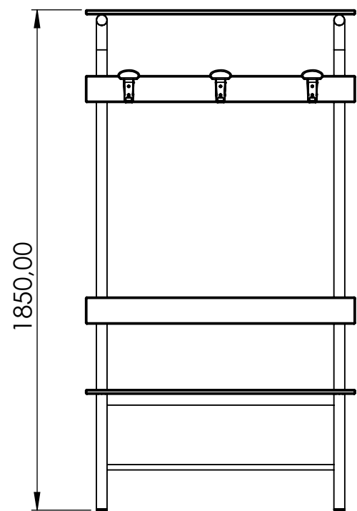
PANCA SPOGLIATOIO CON SCHIENALE, APPENDIABITI E PIANOBORSE CHANGING ROOM BENCH WITH BACKREST, CLOTHES RAIL AND BAG SHELF
