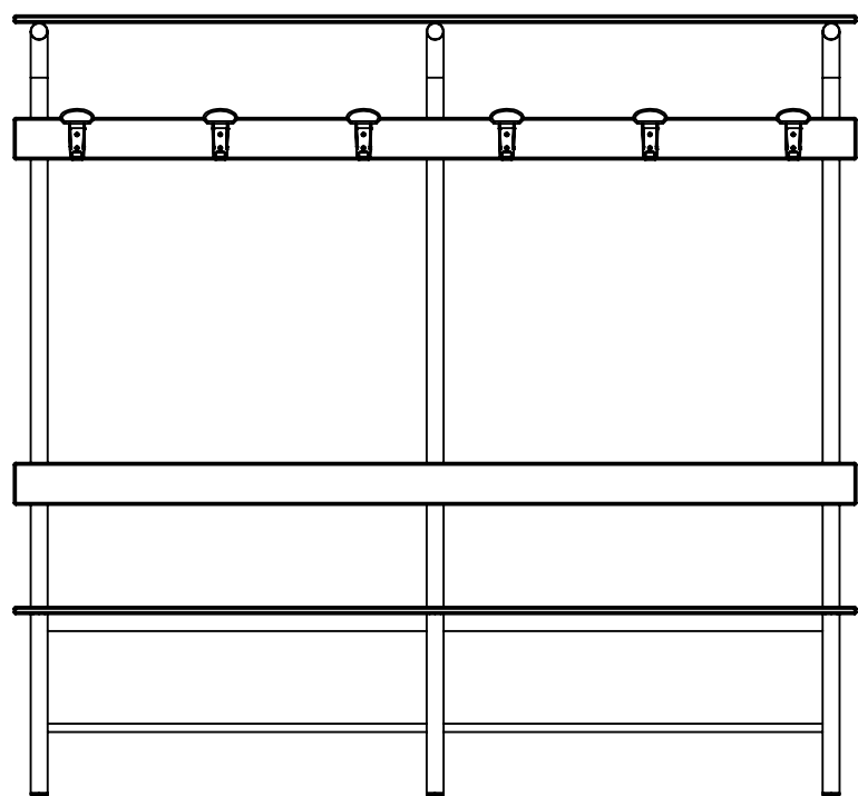
PANCA SPOGLIATOIO CON SCHIENALE, APPENDIABITI E PIANOBORSE CHANGING ROOM BENCH WITH BACKREST, CLOTHES RAIL AND BAG SHELF
