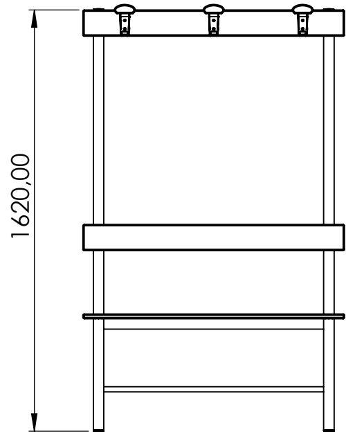
PANCA SPOGLIATOIO CON SCHIENALE E APPENDIABITI CHANGING ROOM BENCH WITH BACKREST AND CLOTHES RAIL
